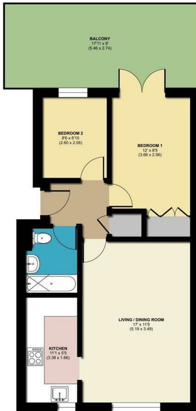
SECOND FLOOR
